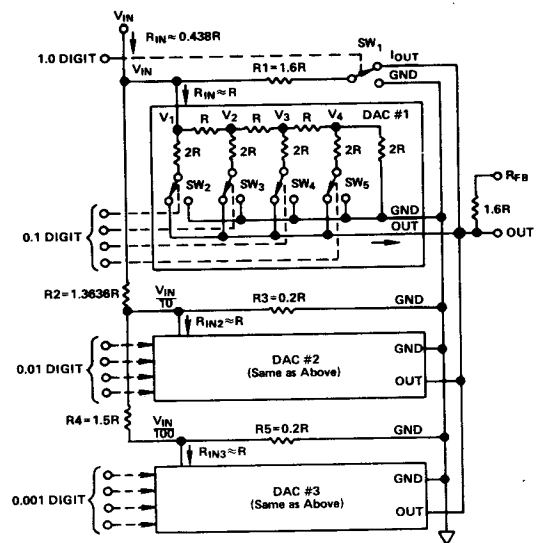
Figure 1. AD7525 Circuit Diagram
