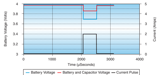
Figure 5. GSM Pulse
