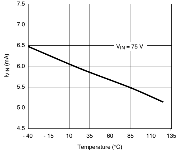
I_{IN} vs. Temperature
