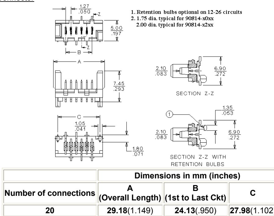
Figure 1. Picoflex Connector
