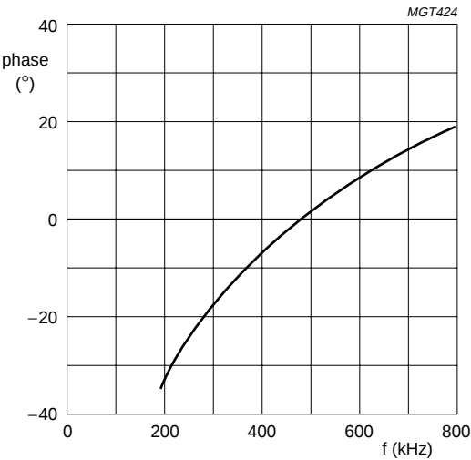
Fig.6 Typical phase of drain ringing at switch-on (at N \times V_o = 80 V).
