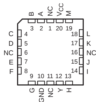
SN54ALS133 . . . FK PACKAGE (TOP VIEW)
