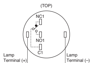
SPDT Contact (Single-pole/Double Throw)
