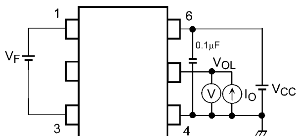
Fig. 13.1.2 I_{OPL} Test Circuit
