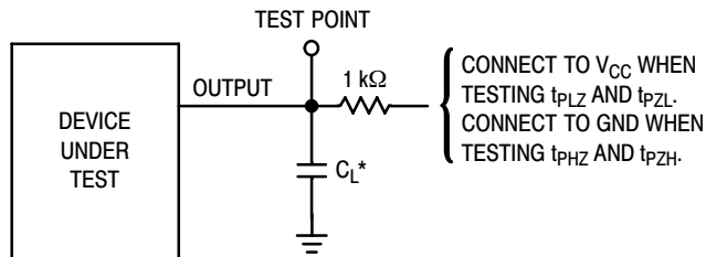
Figure 6. Test Circuit
