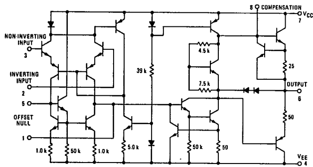
FIGURE 1 - CIRCUIT SCHEMATIC
