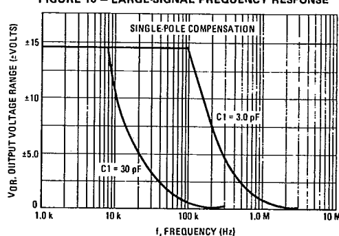
FIGURE 10 - LARGE-SIGNAL FREQUENCY RESPONSE
