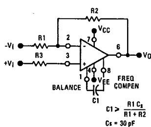
FIGURE 3 - SINGLE-POLE COMPENSATION
