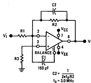
FIGURE 4 - FEEDFORWARD COMPENSATION
