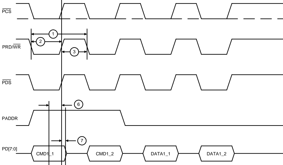
Figure 11. GPI 8-Bit Write Access Using Combined Read/Write and Data Strokes
