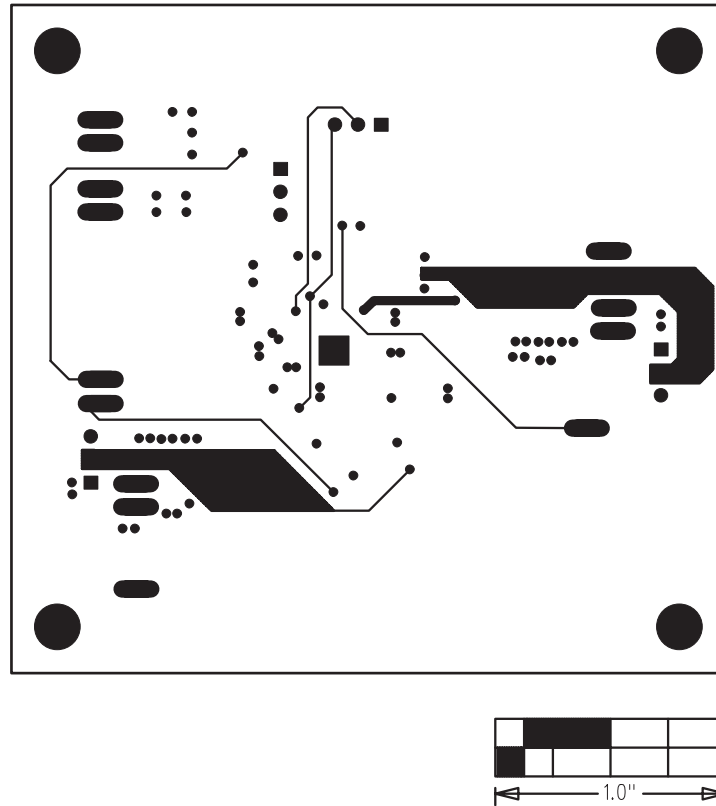
Figure 5. MAX15022 EV Kit PCB Layout—Inner Trace Layer 3
