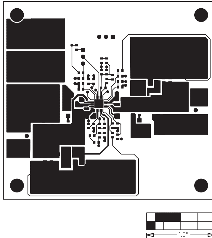
Figure 3. MAX15022 EV Kit PCB Layout—Component Side
