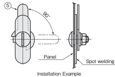
Installation Example
