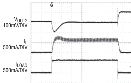
Channel 2 Load Step Response
