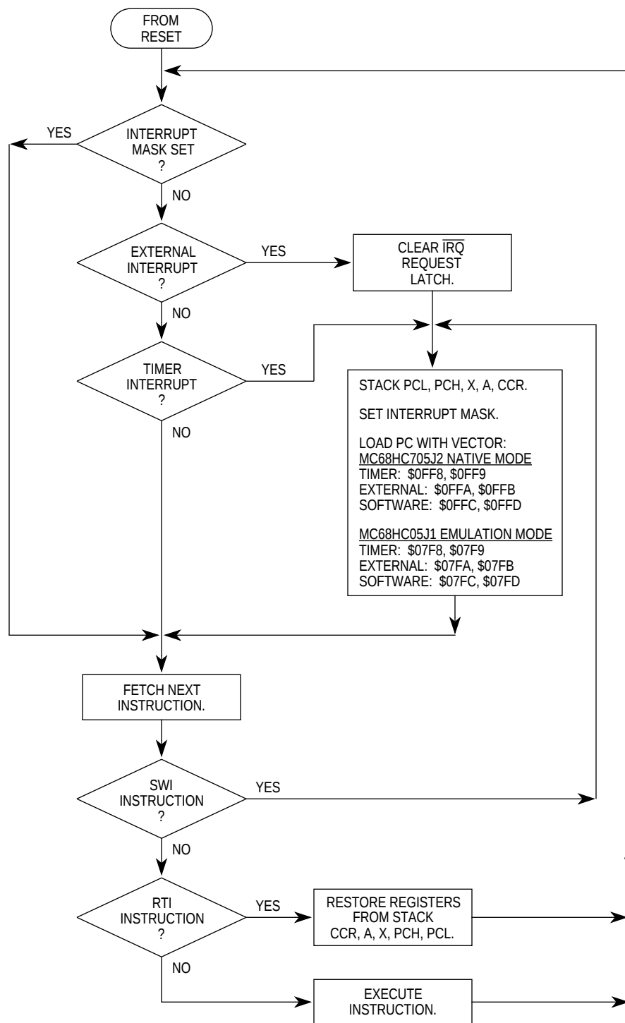
Figure 5-3. Interrupt Flowchart
