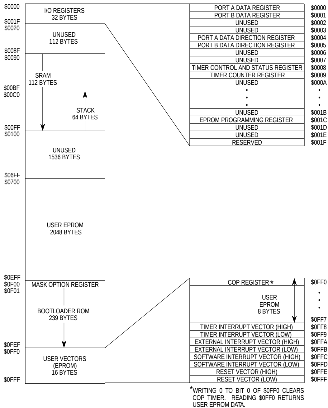
Figure 6-1. Memory Map
