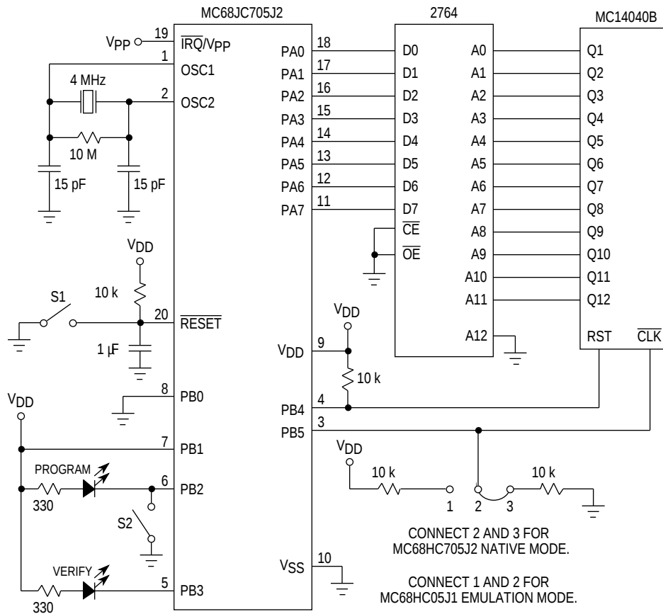
Figure 8-1. Bootloader Circuit
