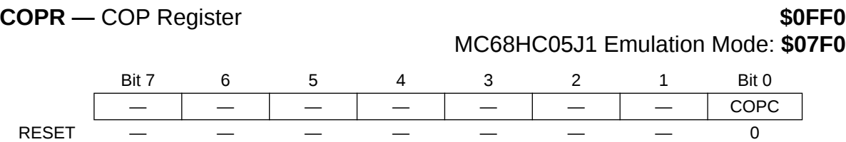
Figure 7-4. COP Register (COPR)
