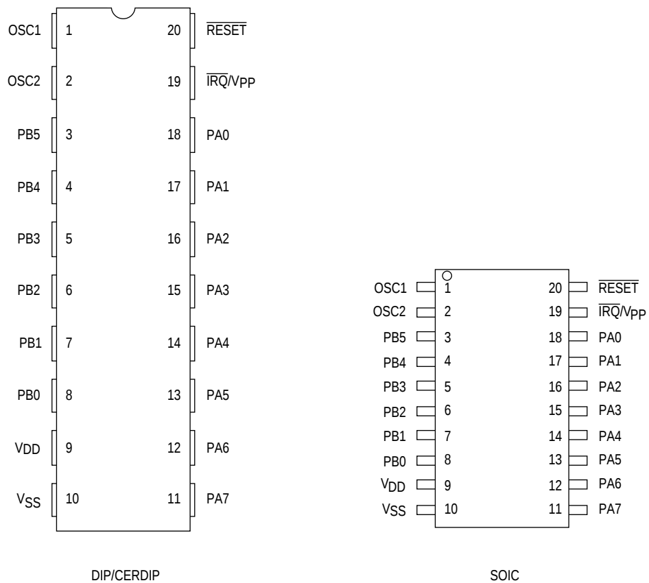
Figure 2-1. Pin Assignments
