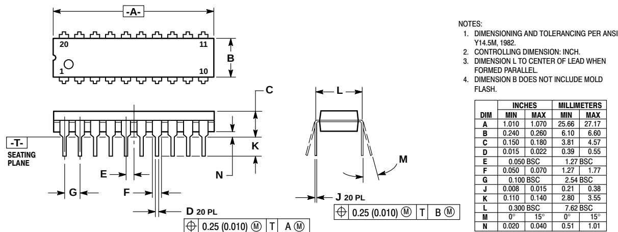
Figure 12-1. MC68HC705J2P (Case 738-03)
