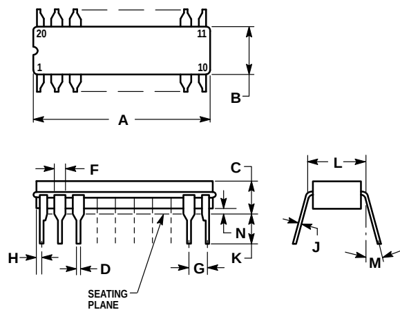
Figure 12-3. MC68HC705J2S (Case 732-03)
