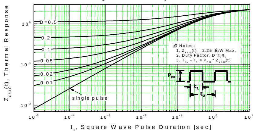
Fig 11. Thermal Response
