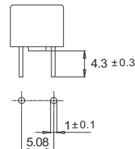
Dimensions [mm]
