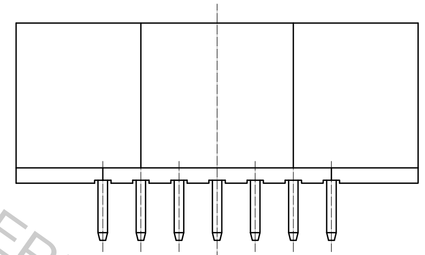
MATING FIGURE (2:1)
