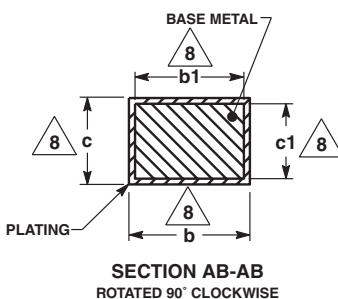
AE SUFFIX (Pb-Free) 64-TERMINAL LQFP EXPOSED PAD PLASTIC PACKAGE 98ARH98426A ISSUE 0
