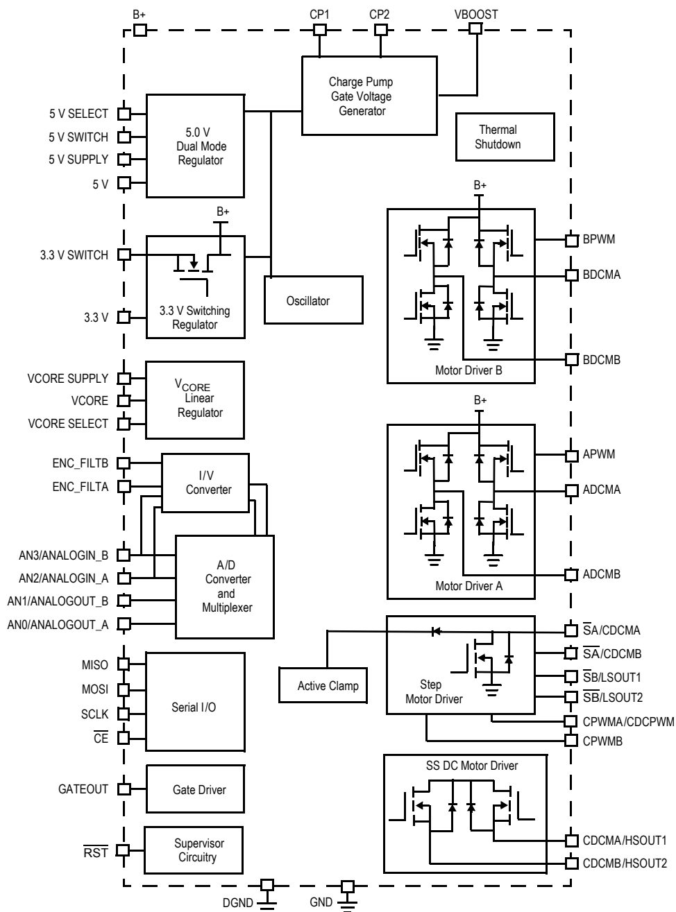
Figure 2. 34921 Simplified Internal Block Diagram
