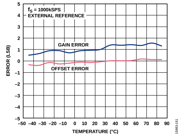
Figure 47. Offset and Gain Errors of the AUX +/-AUX- ADC Channel Pair vs. Temperature
