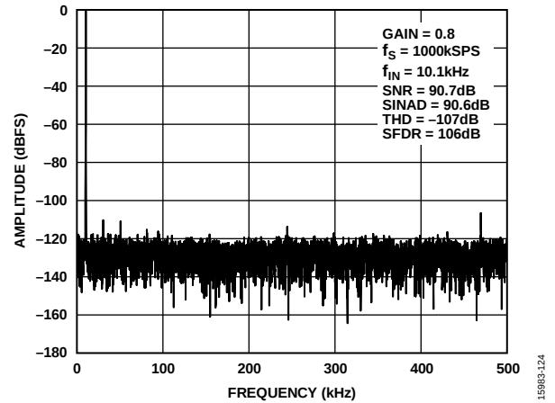
Figure 21. 10 kHz FFT, PGIA Gain = 0.8
