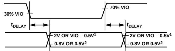
Figure 3. Voltage Levels for Timing
