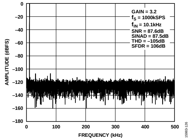
Figure 23. 10 kHz FFT, PGIA Gain = 3.2
