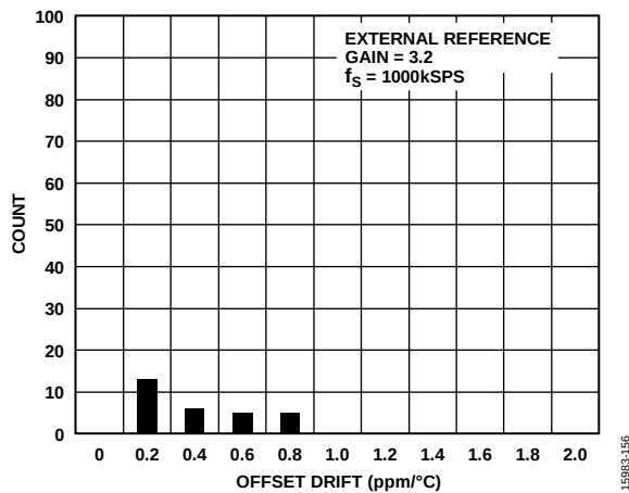
Figure 14. Offset Drift, PGIA Gain = 3.2
