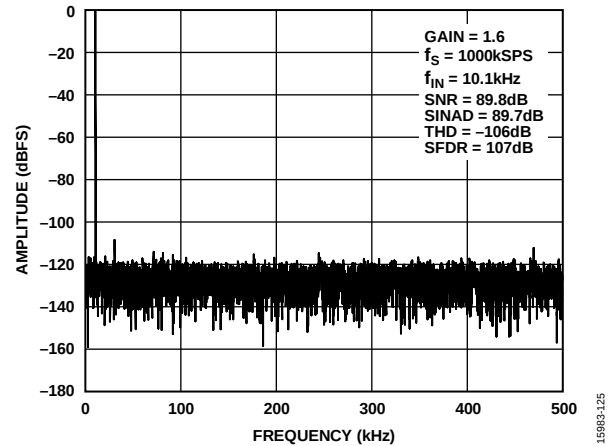
Figure 22. 10 kHz FFT, PGIA Gain = 1.6
