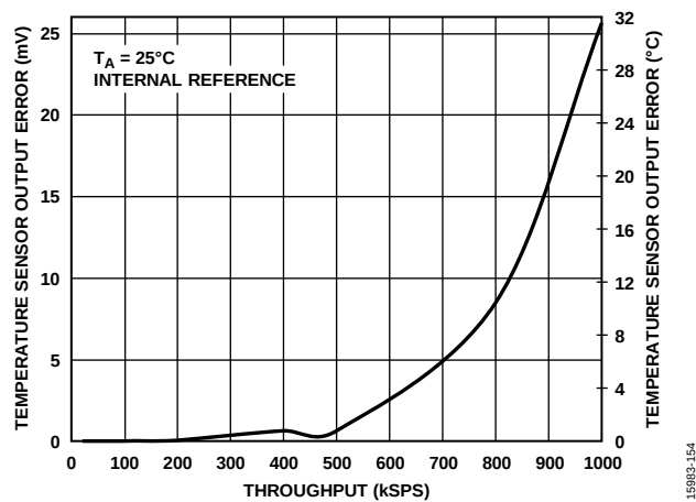
Figure 50. Temperature Sensor Output Error vs. Throughput
