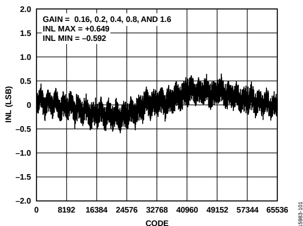
Figure 6. Integral Nonlinearity (INL) vs. Code, PGIA Gain = 0.16, 0.2, 0.4, 0.8, and 1.6
