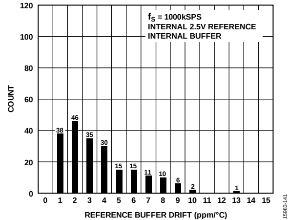
Figure 17. Reference Buffer Drift, Internal 2.5 V Reference
