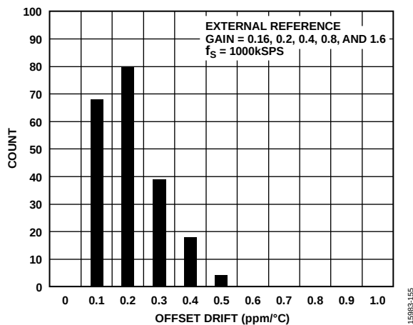
Figure 13. Offset Drift, PGIA Gain = 0.16, 0.2, 0.4, 0.8, and 1.6
