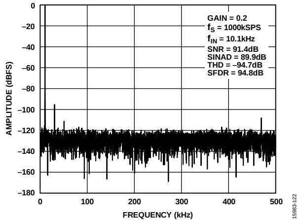
Figure 19. 10 kHz FFT, PGIA Gain = 0.2
