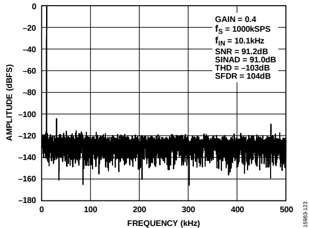
Figure 20. 10 kHz FFT, PGIA Gain = 0.4
