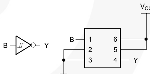
Figure 7. Inverter
