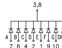
POLARITY DIAGRAM
