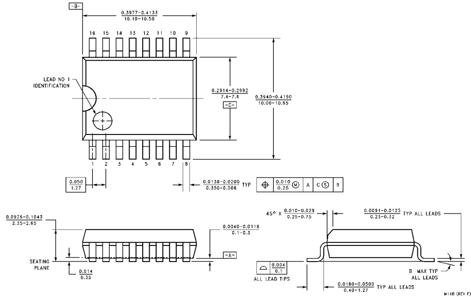
16-Lead Small Outline Integrated Circuit (SOIC), JEDEC MS013, 0.300" Wide Body Package Number M16B
