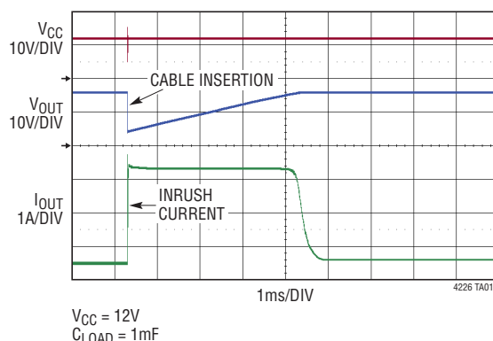
Inrush after Load Connection
