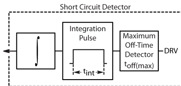
Figure 11. Output Short-Circuit Detector
