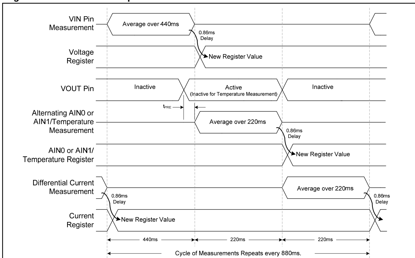
Figure 4. Measurement Sequence
