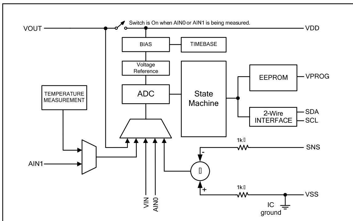
Figure 2. Block Diagram
