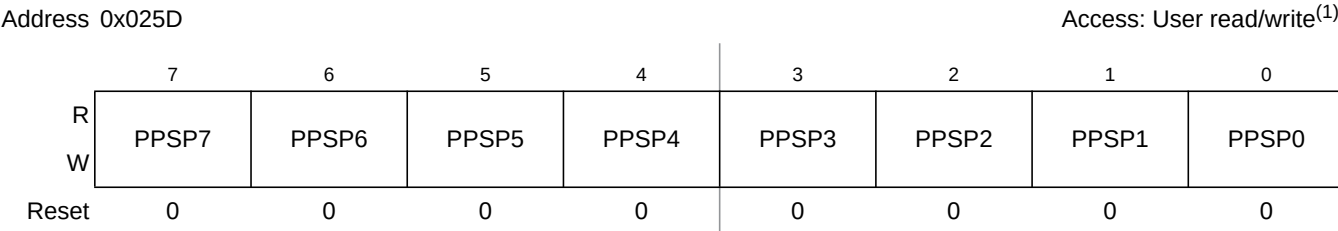
Figure 19-48. Port P Polarity Select Register (PPSP)
