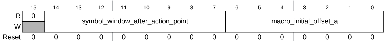
Figure 13-71. Protocol Configuration Register 6 (PCR6)
