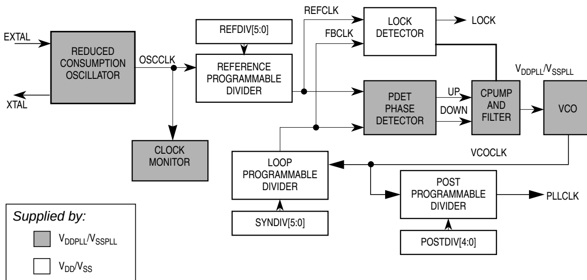
Figure 2-15. IPLL Functional Diagram
