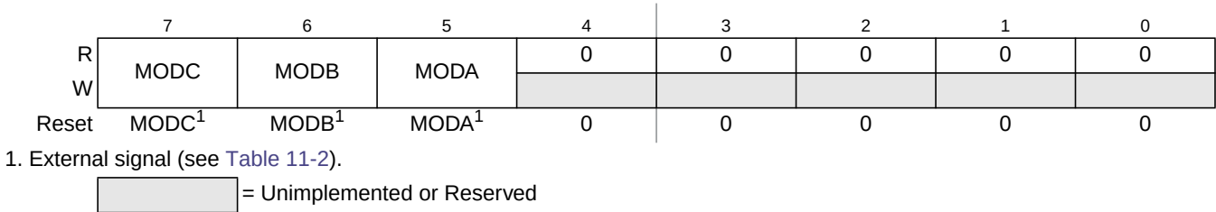
Figure 11-4. Mode Register (MODE)
