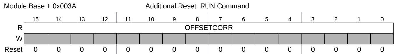
Figure 13-29. Offset Correction Value Register (OFCORVR)
