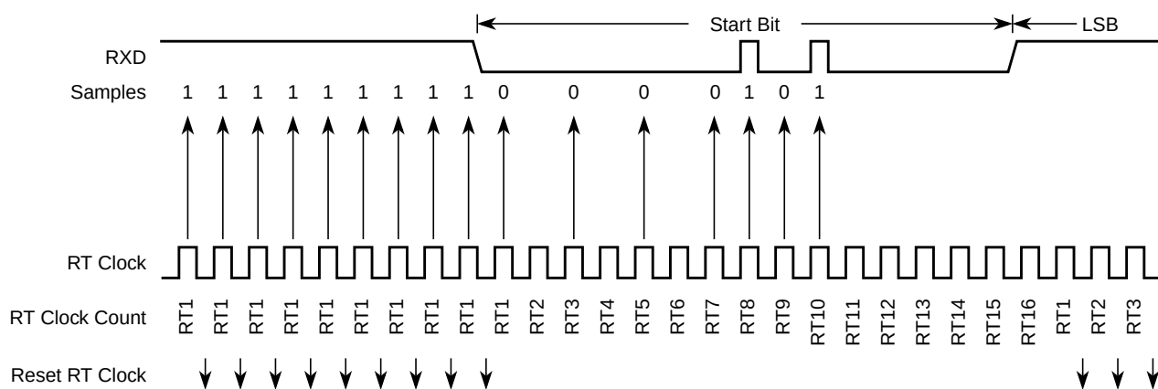
In Figure 23-27 , a noise burst makes the majority of data samples RT8, RT9, and RT10 high. This sets the noise flag but does not reset the RT clock. In start bits only, the RT8, RT9, and RT10 data samples are ignored.
