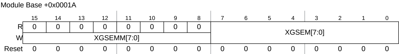
Figure 14-12. XGATE Semaphore Register (XGSEM)
