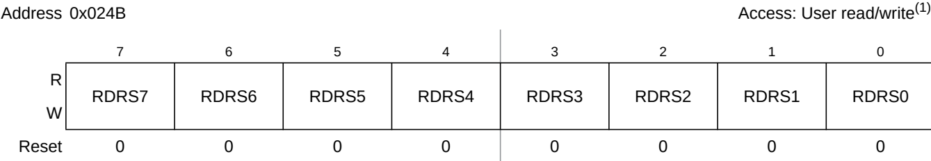
Figure 19-30. Port S Reduced Drive Register (RDRS)
