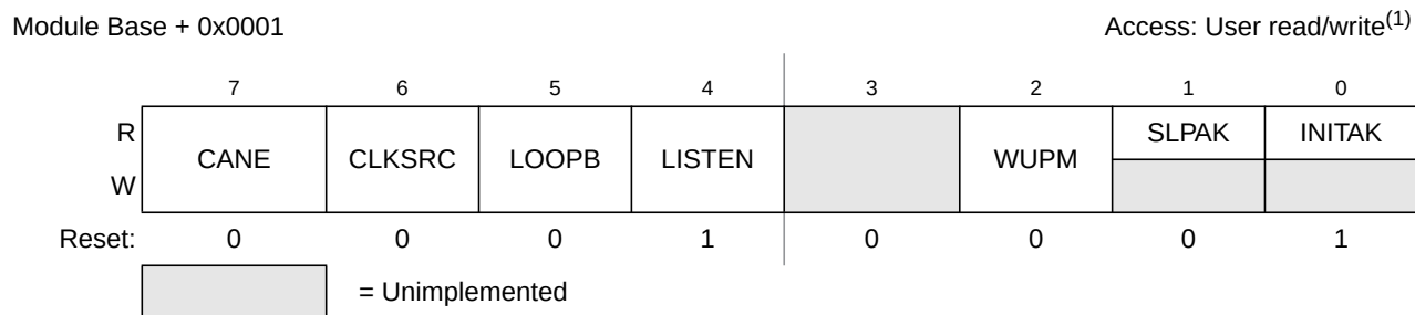
Figure 21-5. MSCAN Control Register 1 (CANCTL1)
