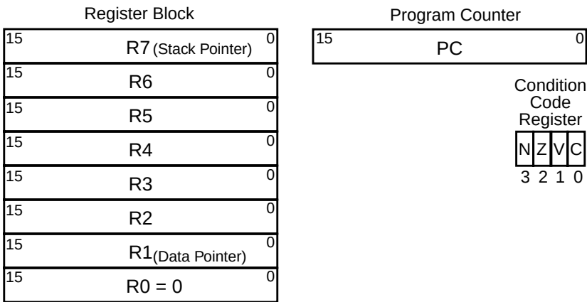
Figure 14-22. Programmer’s Model
