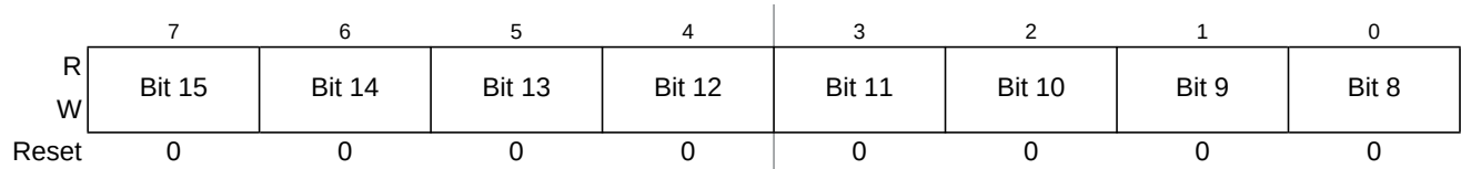
Figure 16-16. Debug Comparator Address Mid Register (DBGXAM)
