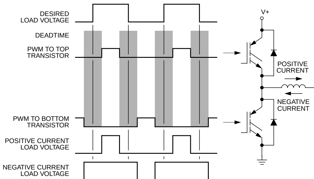
Figure 20-53. Deadtime Distortion
