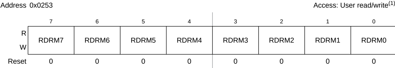
Figure 19-38. Port M Reduced Drive Register (RDRM)
