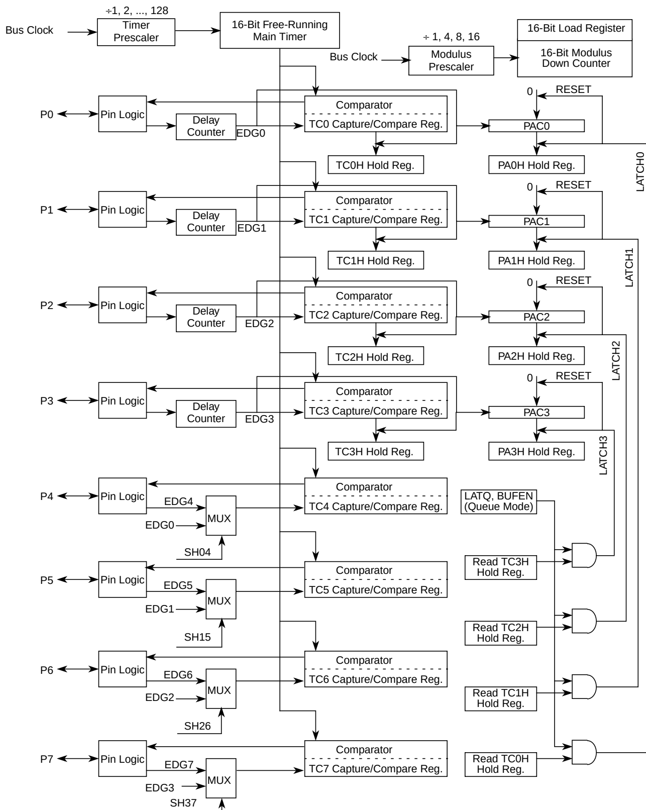
Figure 26-69. Detailed Timer Block Diagram in Queue Mode when PRNT = 0
