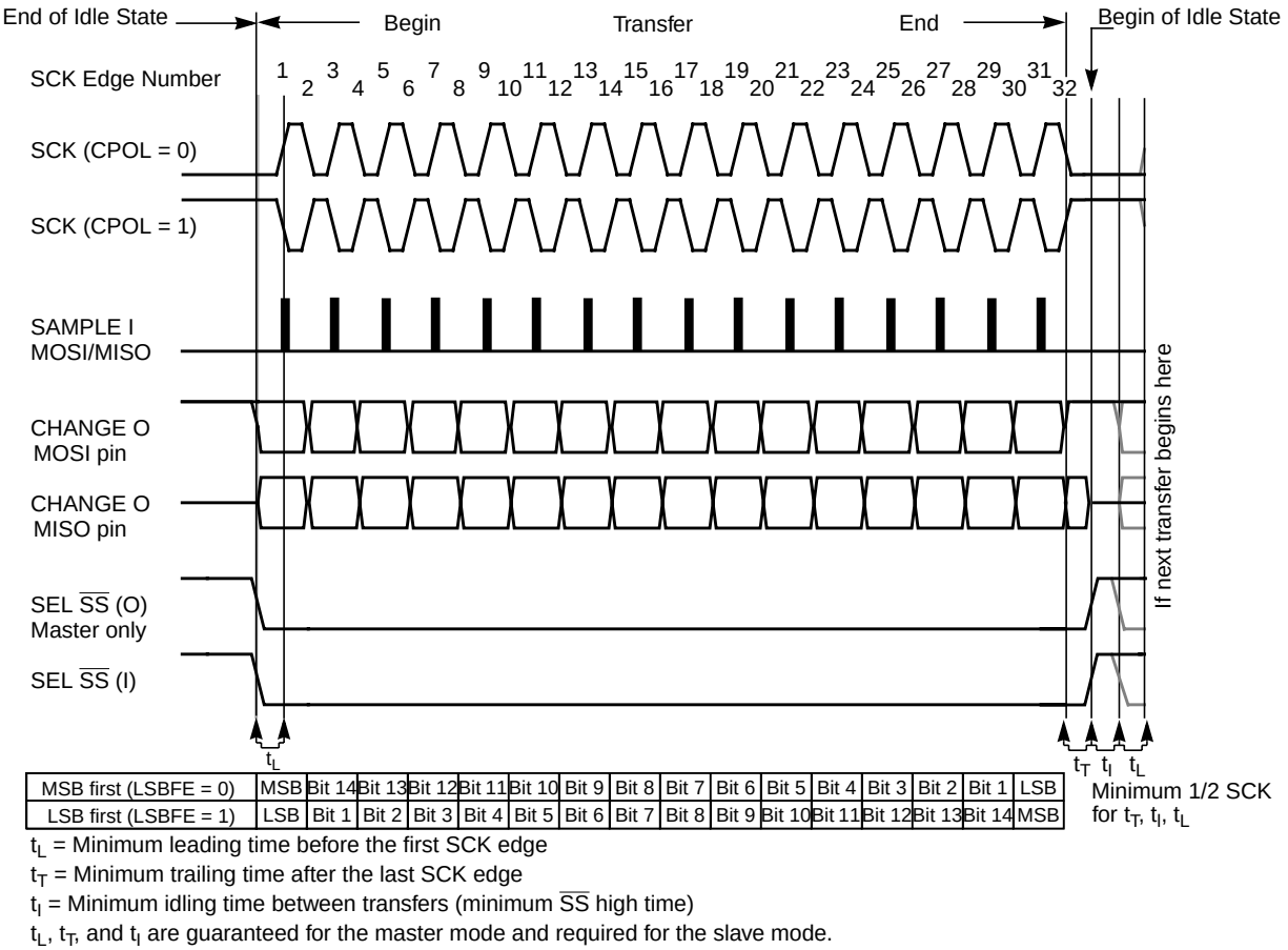
Figure 25-13. SPI Clock Format 0 (CPHA = 0), with 16-Bit Transfer Width selected (XFRW = 1)
