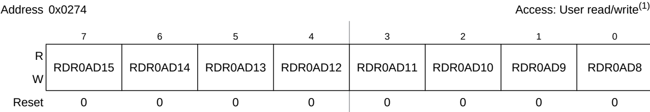
Figure 19-71. Port AD Reduced Drive Register 0 (RDR0AD)
