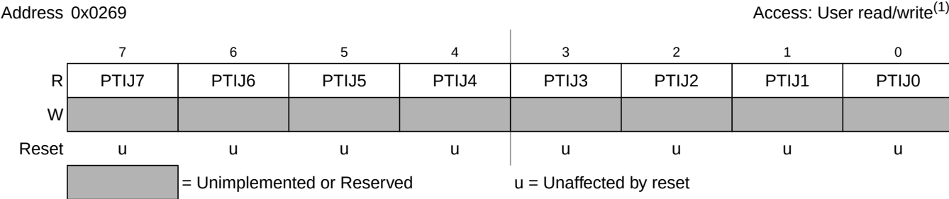
Figure 19-60. Port J Input Register (PTIJ)
