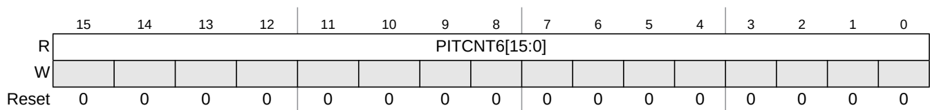
Figure 22-25. PIT Count Register 6 (PITCNT6)
