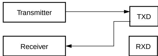
Figure 23-30. Single-Wire Operation (LOOPS = 1, RSRC = 1)
