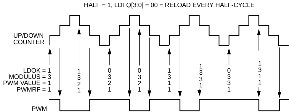
Figure 20-70. Half-Cycle Center-Aligned PWM Value Loading
