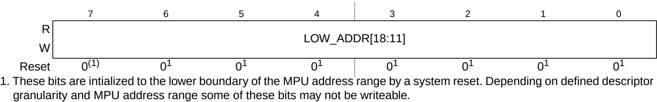
Figure 17-9. MPU Descriptor Register 1 (MPUDESC1)
