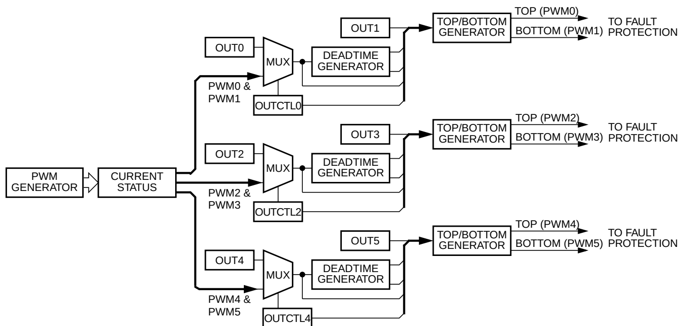
Figure 20-49. Deadtime Generators
