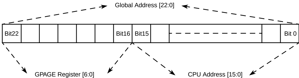
Figure 11-7. GPAGE Address Mapping
