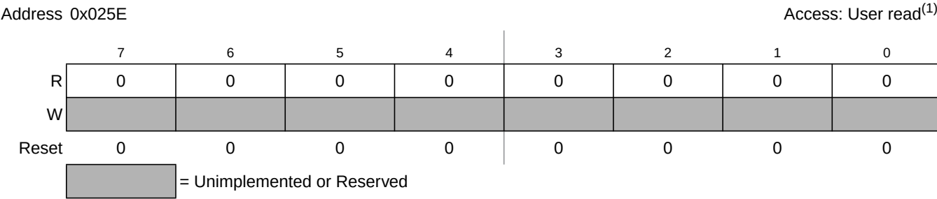
Figure 19-49. PIM Reserved Register
