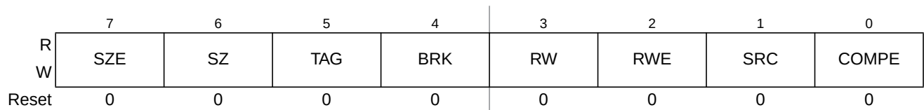
Figure 16-14. Debug Comparator Control Register (Comparators B and D)
