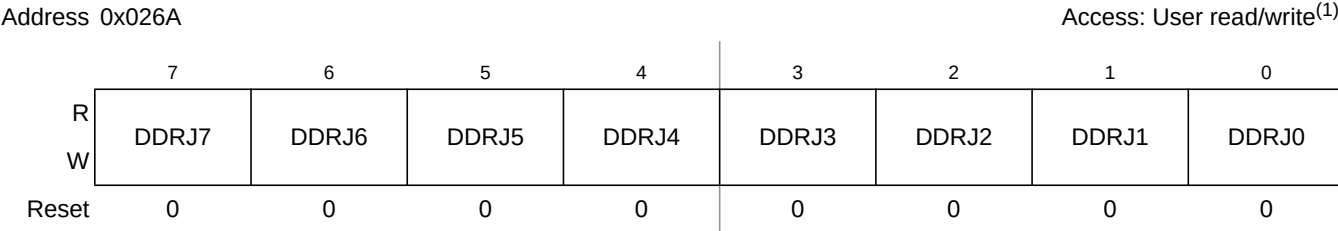
Figure 19-61. Port J Data Direction Register (DDRJ)
