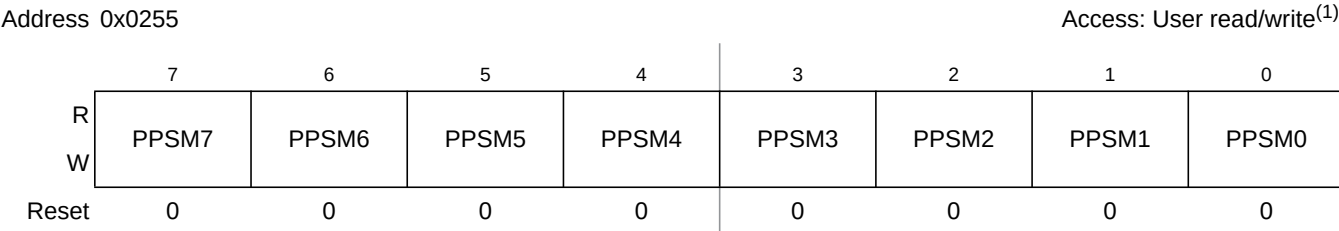
Figure 19-40. Port M Polarity Select Register (PPSM)
