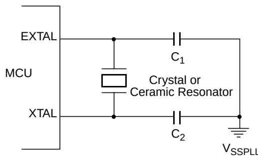
Figure 1-9. Loop Controlled Pierce Oscillator Connections ( \overline{\text{XCLKS}} = 1 )
