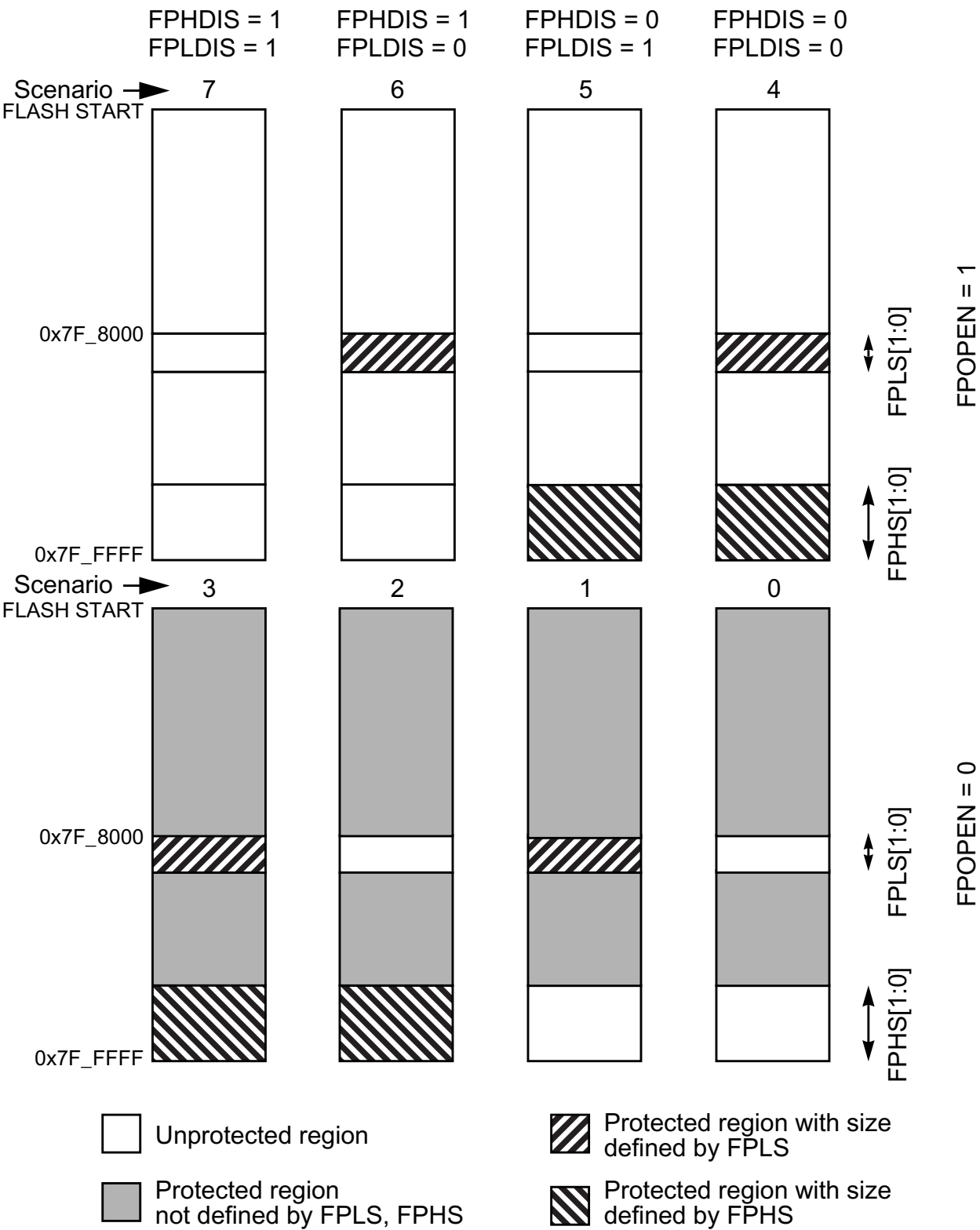
Figure 9-14. P-Flash Protection Scenarios
