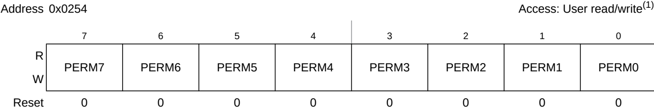
Figure 19-39. Port M Pull Device Enable Register (PERM)
