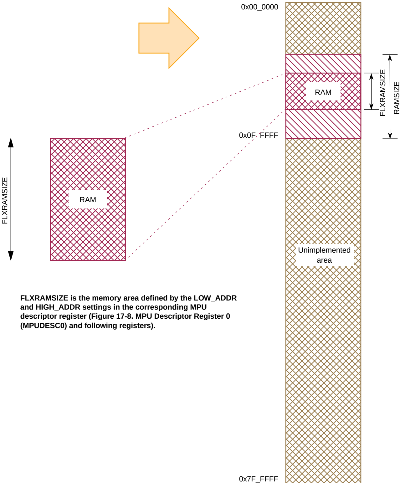
Figure 1-4. FLEXRAY Global Address Mapping
