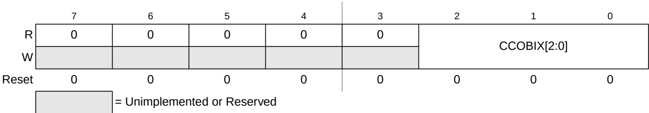
Figure 9-7. FCCOB Index Register (FCCOBIX)
