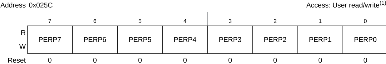
Figure 19-47. Port P Pull Device Enable Register (PERP)
