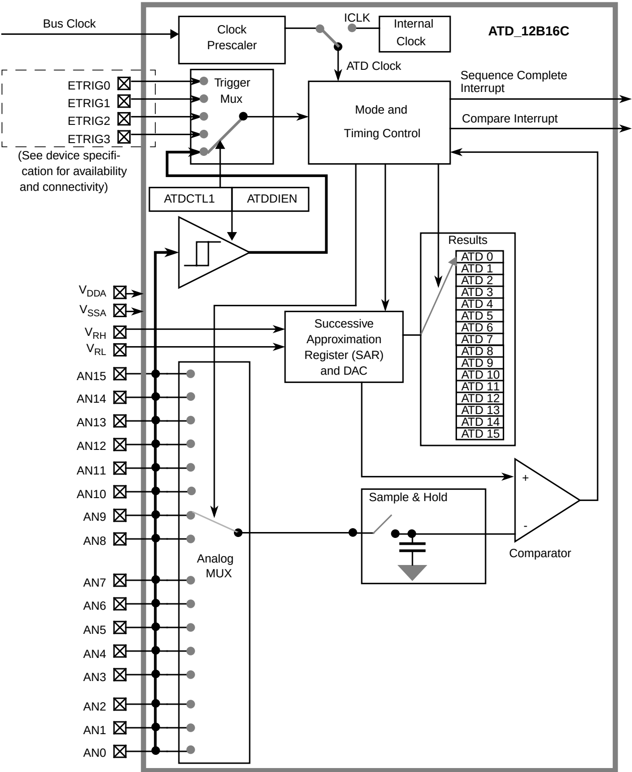
Figure 24-1. ADC12B16C Block Diagram
