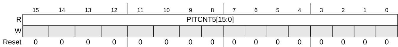
Figure 22-24. PIT Count Register 5 (PITCNT5)
