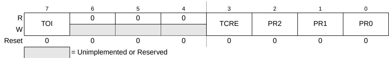
Figure 26-16. Timer System Control Register 2 (TSCR2)
