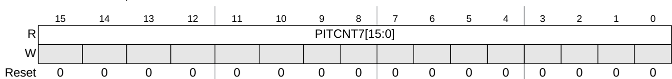
Figure 22-26. PIT Count Register 7 (PITCNT7)
