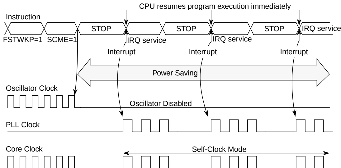
Figure 2-19. Fast Wake-up from Full Stop Mode: Example 1
