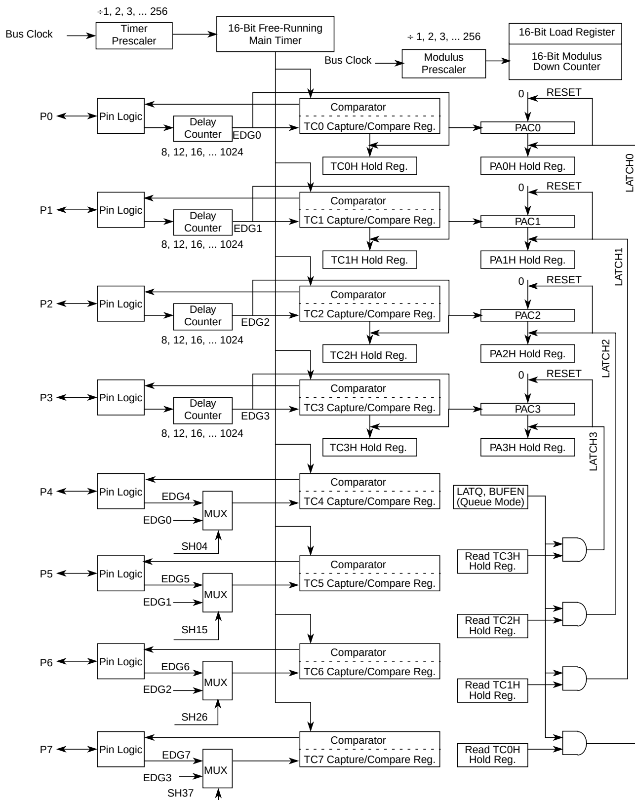
Figure 26-70. Detailed Timer Block Diagram in Queue Mode when PRNT = 1
