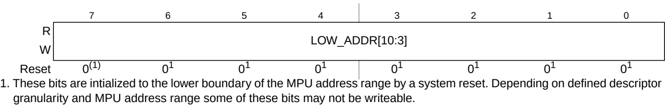
Figure 17-10. MPU Descriptor Register 2 (MPUDESC2)
