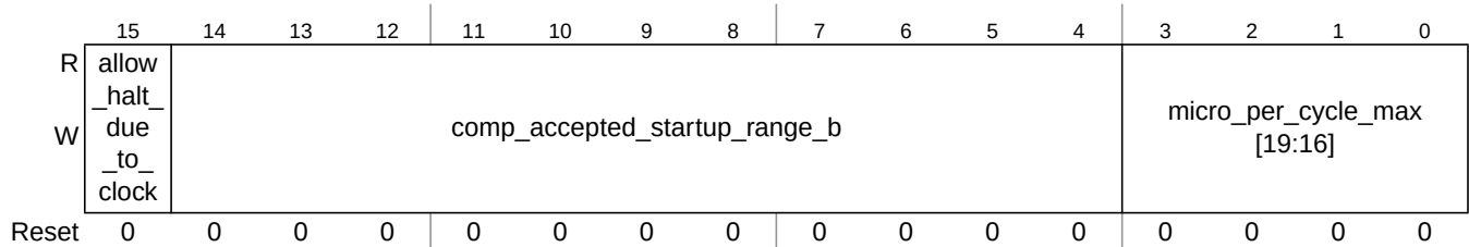
Figure 13-91. Protocol Configuration Register 26 (PCR26)
