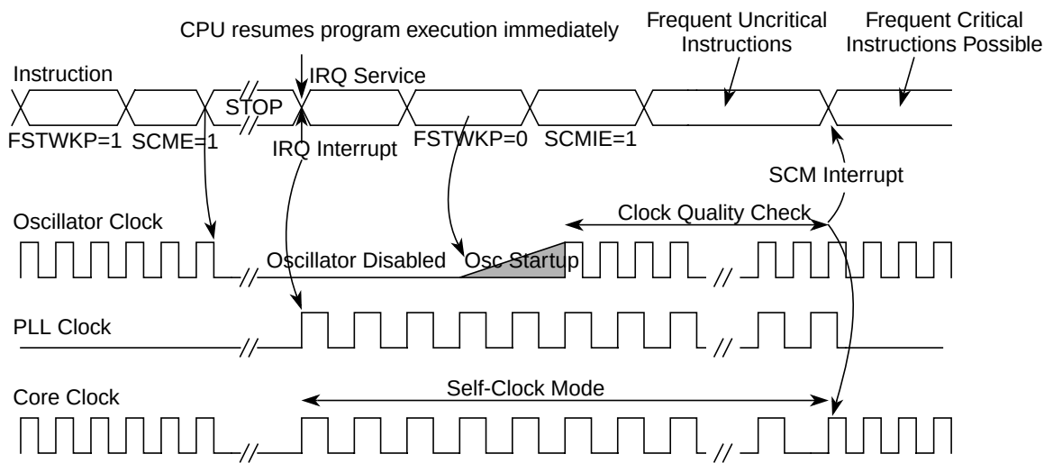
Figure 2-20. Fast Wake-up from Full Stop Mode: Example 2
