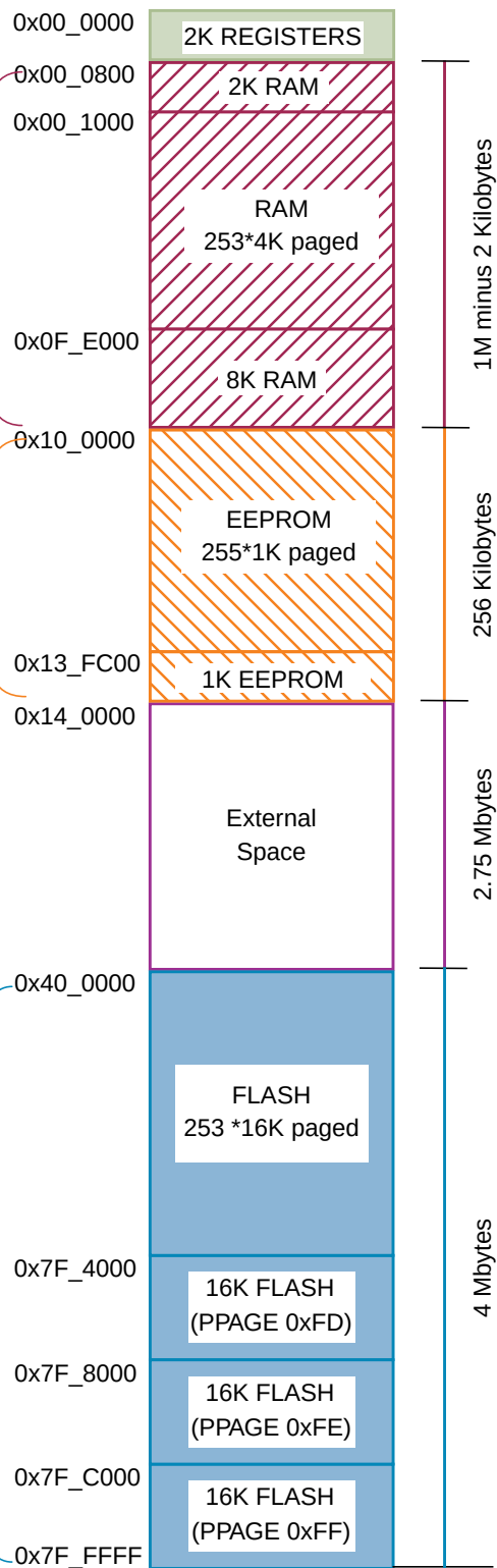
Figure 11-17. Expansion of the Local Address Map
