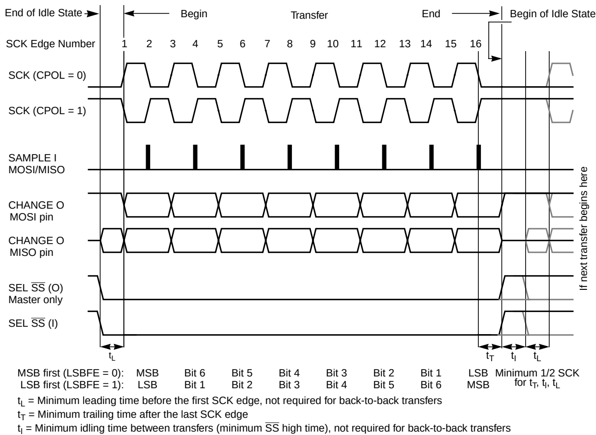
Figure 25-14. SPI Clock Format 1 (CPHA = 1), with 8-Bit Transfer Width selected (XFRW = 0)
