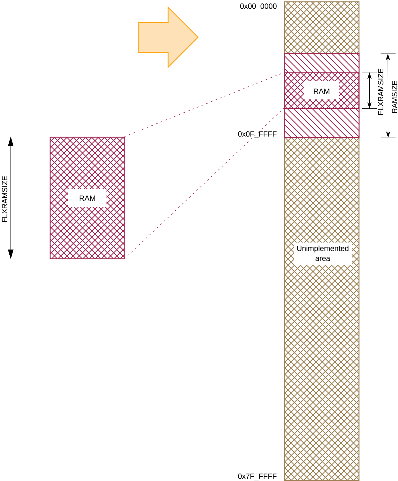
Figure 11-20. FLEXRAY Global Address Mapping
