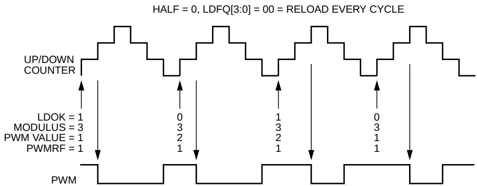
Figure 20-68. Full-Cycle Center-Aligned PWM Value Loading
