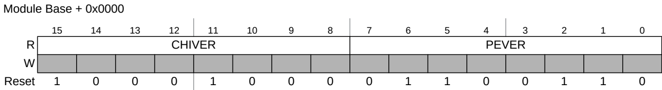
Figure 13-2. Module Version Register (MVR)
