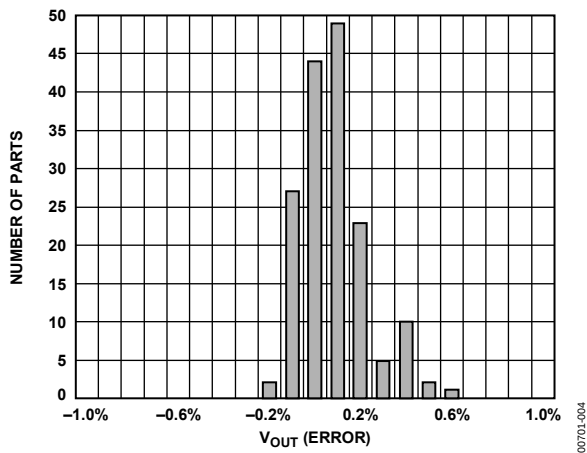
Figure 4. Typical Output Voltage Error Distribution
