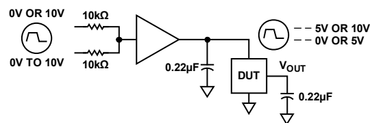
Figure 21. Turn-On/Transient Response Test Circuit
