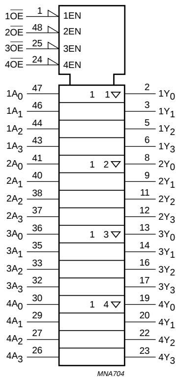
Fig.4 Logic symbol (IEEE/IEC).
