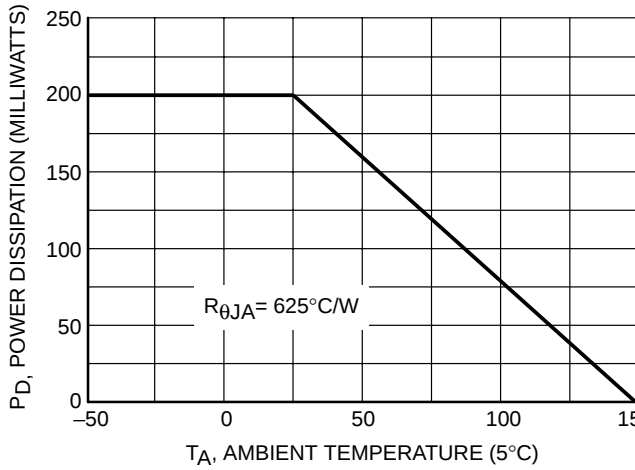
Figure 1. Derating Curve
