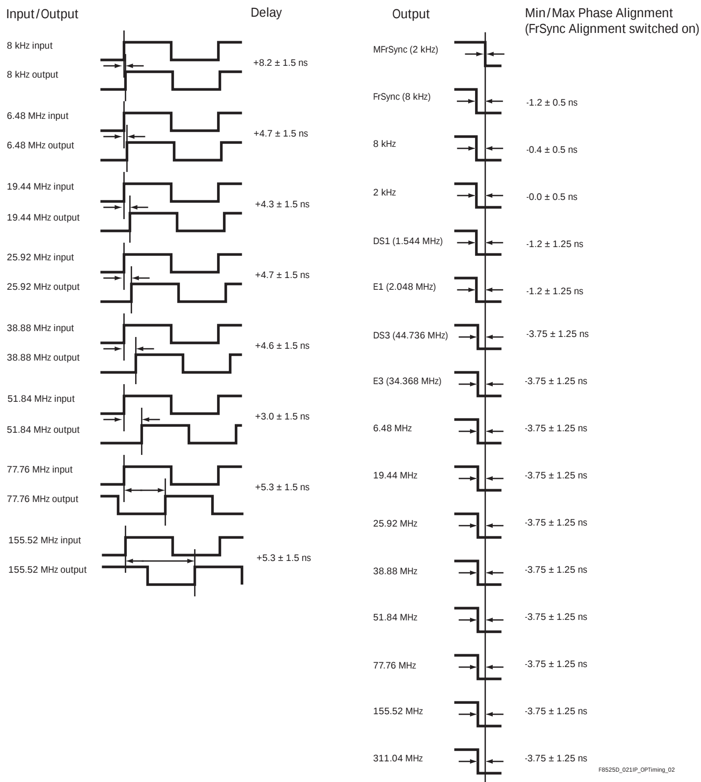
Figure 28 Input/Output Timing
