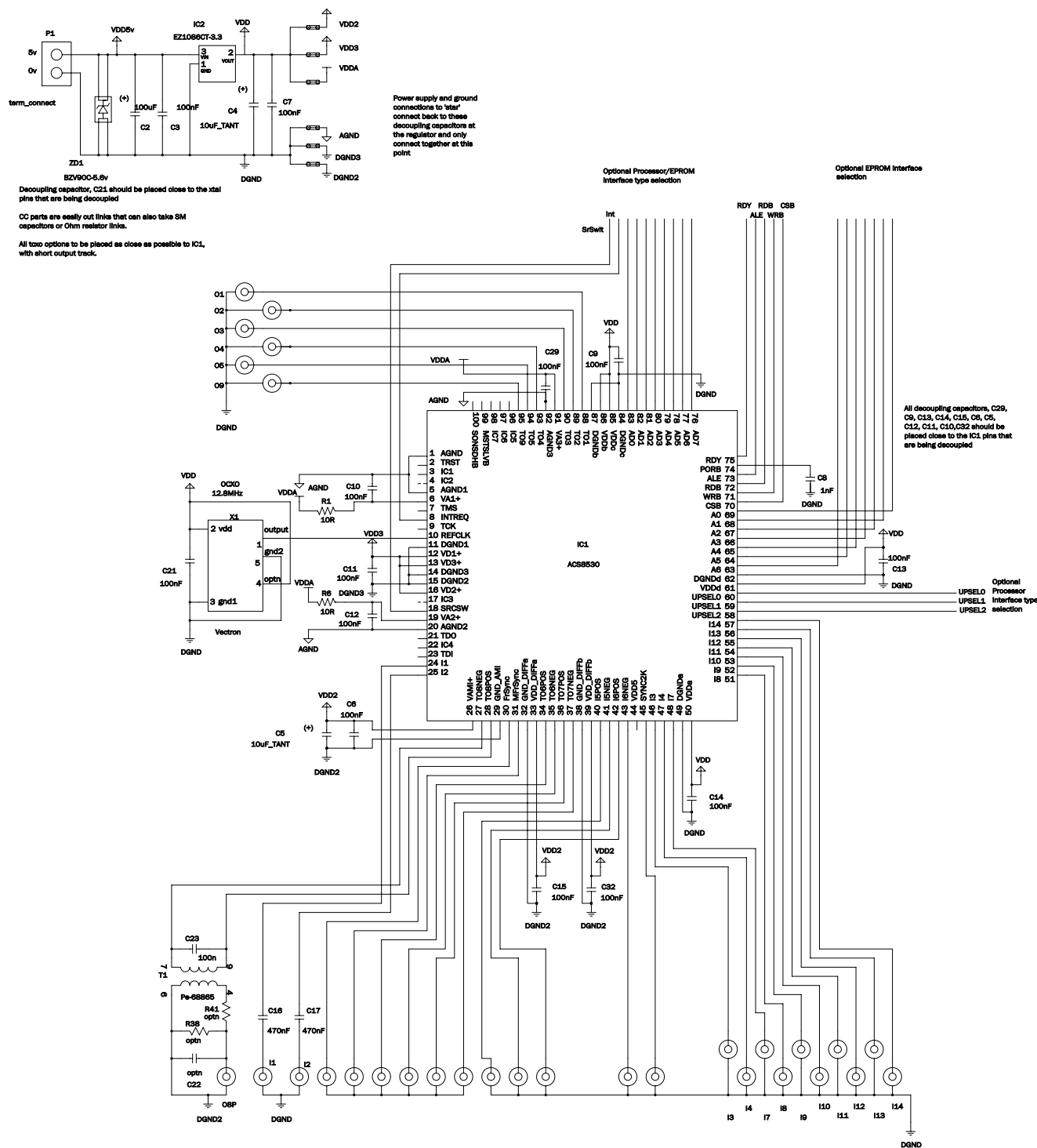
Figure 31 Simplified Application Schematic
