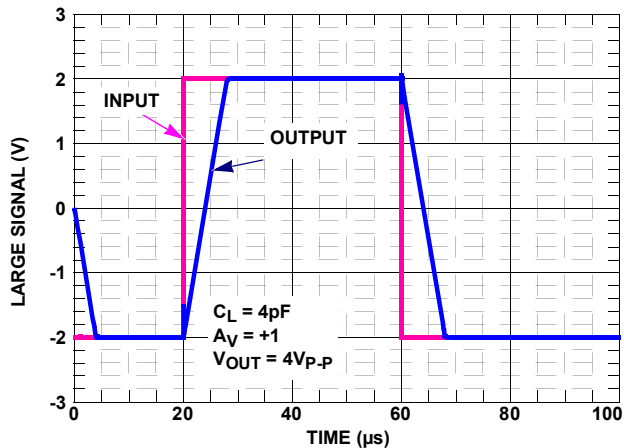
FIGURE 65. SIMULATED LARGE SIGNAL 10V STEP RESPONSE
