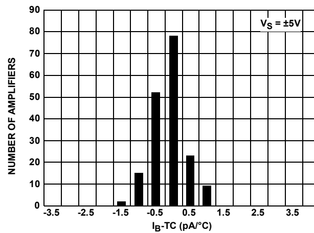
FIGURE 18. TCI_{B-} vs NUMBER OF AMPLIFIERS
