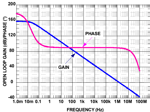
FIGURE 67. SIMULATED OPEN-LOOP GAIN, PHASE vs FREQUENCY
