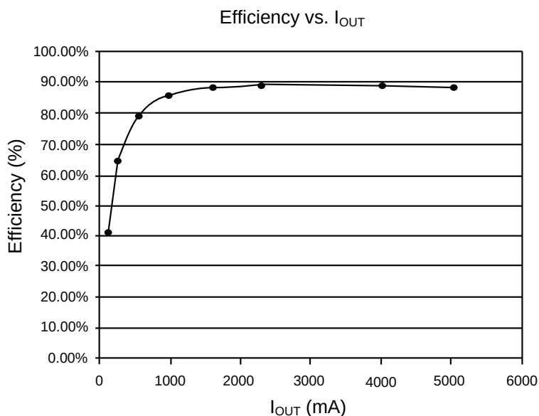
Figure 10 · Output Efficiency @ V_{OUT}=5V , V_{IN}=12V
