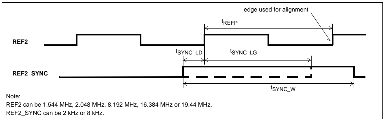
Figure 27 - REF2_SYNC Timing
