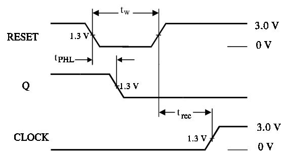
Figure 2. Switching Waveforms
