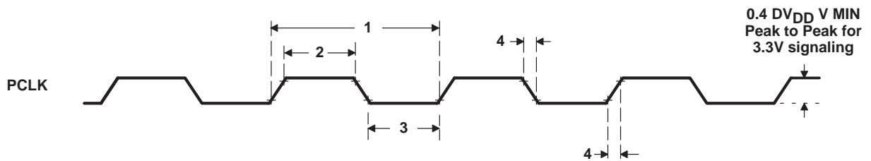
Figure 42. PCLK Timing
