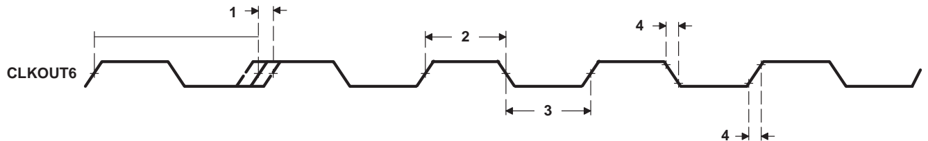
Figure 13. CLKOUT6 Timing
