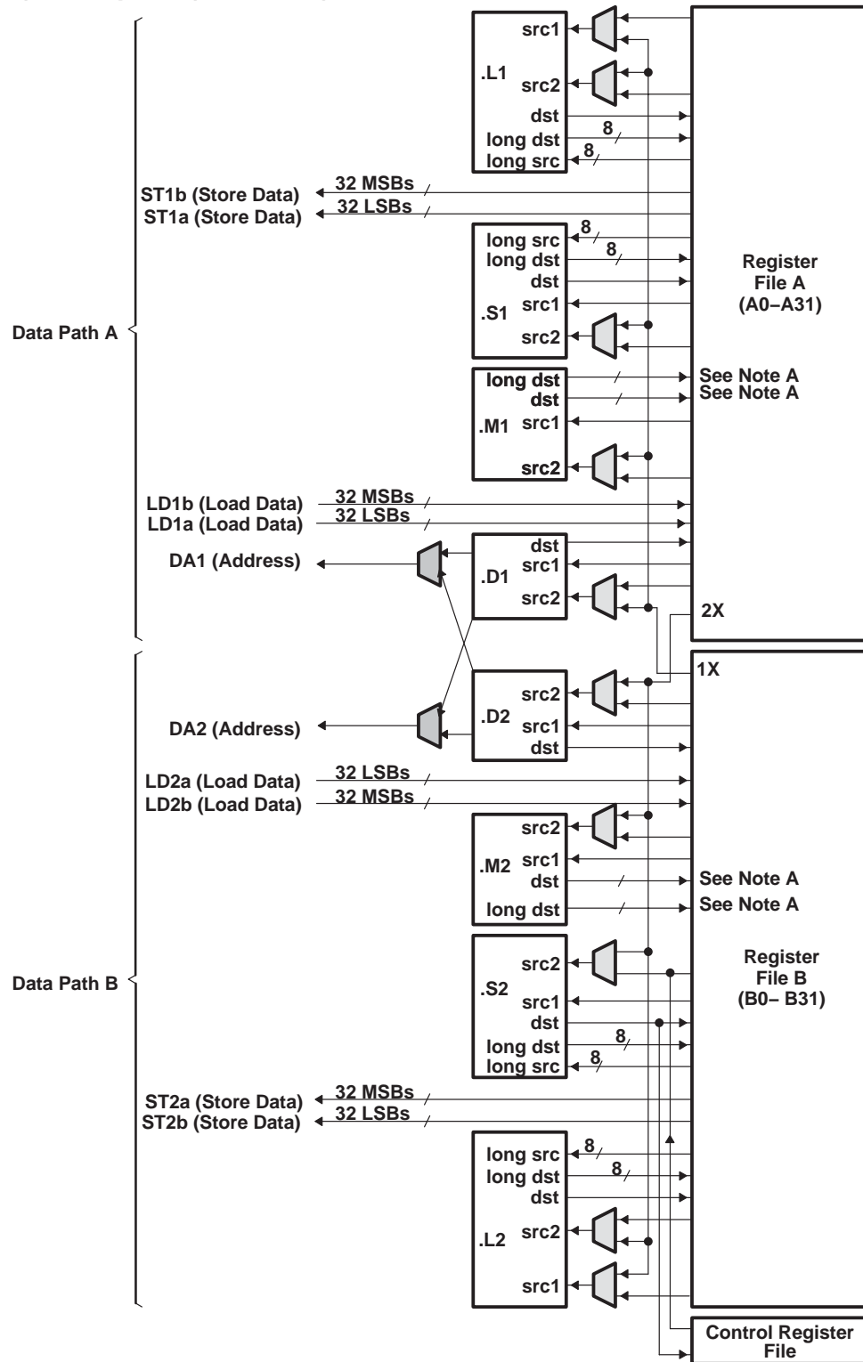
Figure 1. SM320C64x™ CPU (DSP Core) Data Paths
