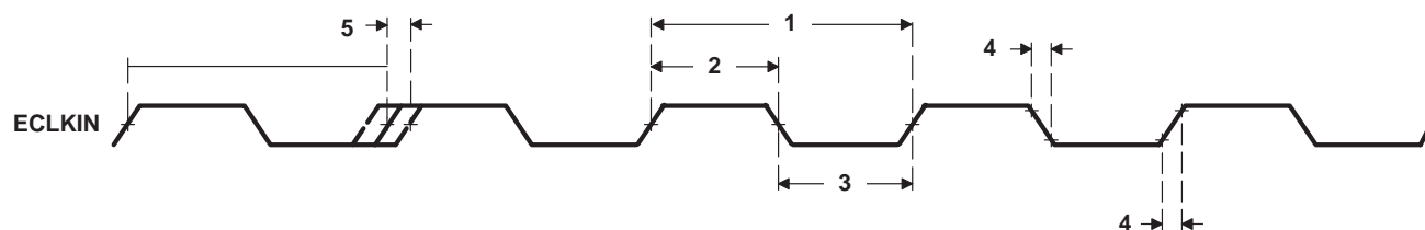
Figure 14. ECLKIN Timing for EMIFA and EMIFB
