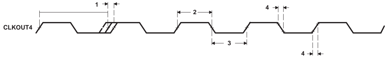
Figure 12. CLKOUT4 Timing
