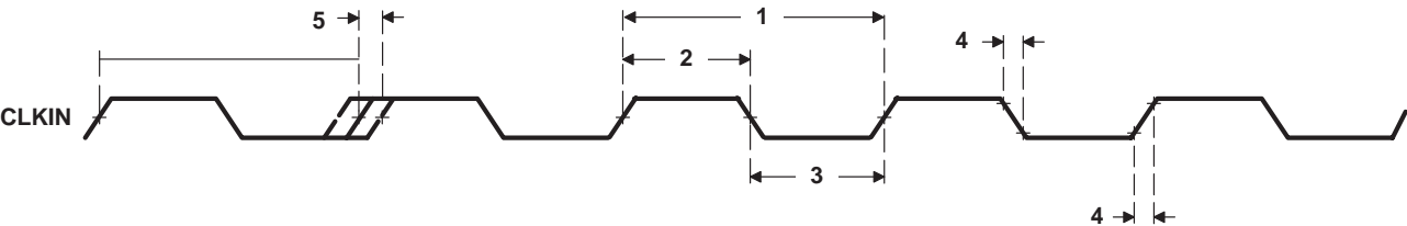
Figure 11. CLKIN Timing
