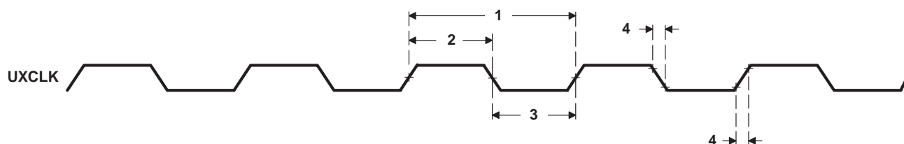
Figure 52. UXCLK Timing
