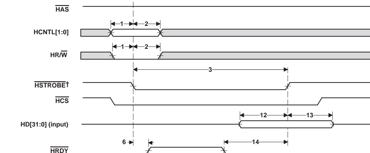
Figure 40. HPI32 Write Timing ( \overline{\text{HAS}} Not Used, Tied High)
