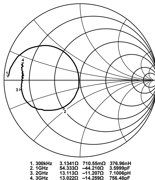
Figure 156. Measured Smith Chart Showing the DAC Output Impedance; f_{DAC} = 2.6 GSFS
