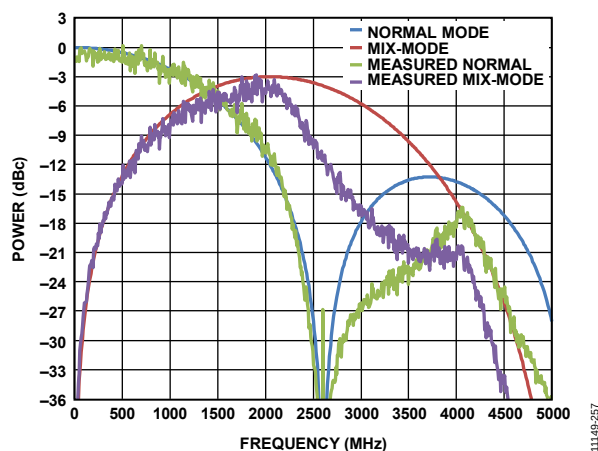
Figure 155. Measured vs. Ideal DAC Output Response; f_{DAC} = 2.6 GSFS
