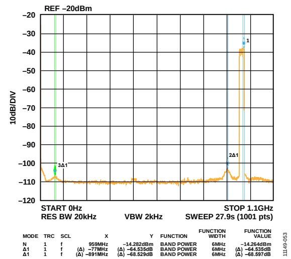
Figure 42. Four Carrier at 950 MHz Output
