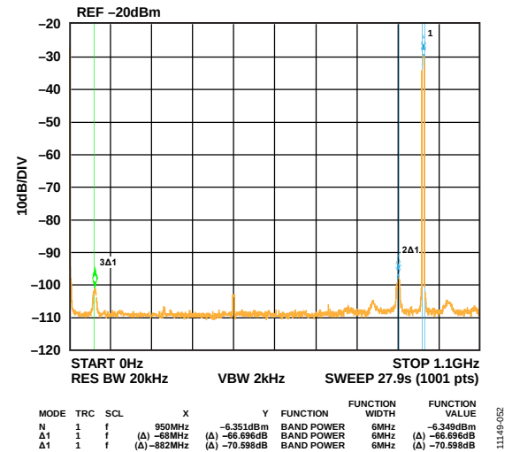
Figure 41. Single Carrier at 950 MHz Output
