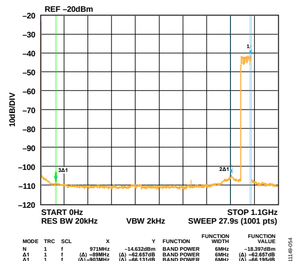
Figure 43. Eight Carrier at 950 MHz Output
