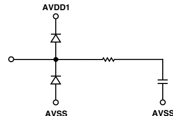
Figure 3. CCDIN (Pin 30)
