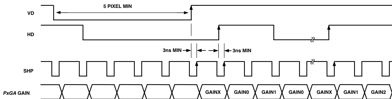
Figure 18. PxGA Mode 6 (Mosaic Repeat) Frame/Line Gain Register Sequence
