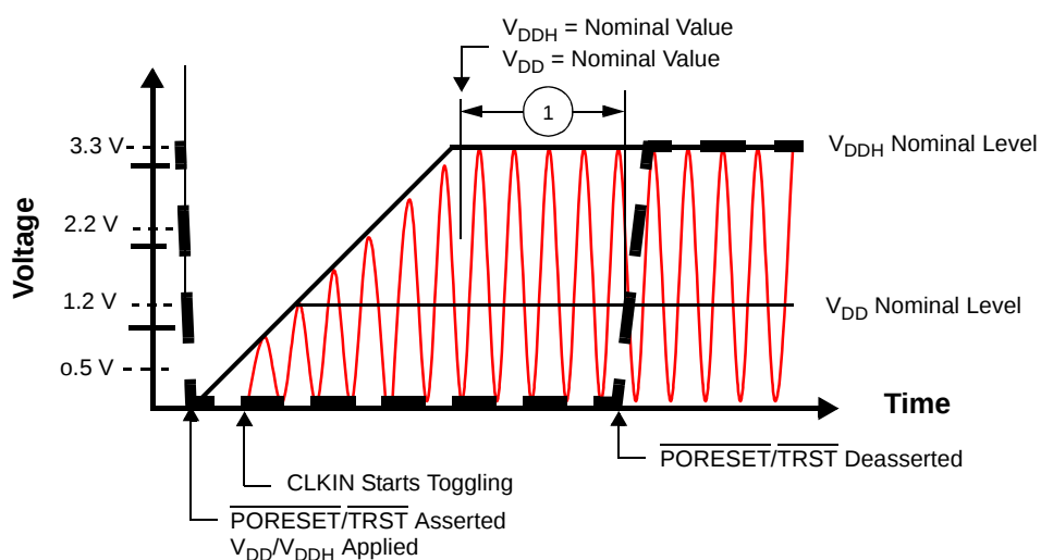
Figure 6. Start-Up Sequence: V_{DD} and V_{DDH} Raised Together
