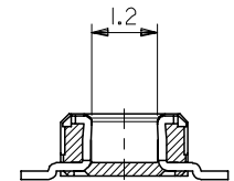
SECT.V-V(W/O LOCK PART)
