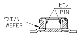
SECT.W-W(LOCK PART)
