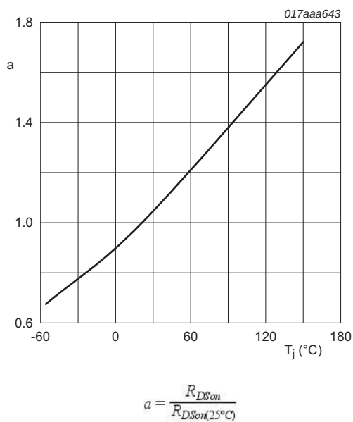
Fig 10. TR1: Normalized drain-source on-state resistance as a function of junction temperature; typical values
