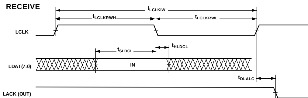
Figure 25. Link Ports—Receive
