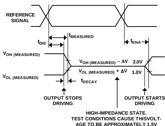
Figure 31. Output Enable/Disable
