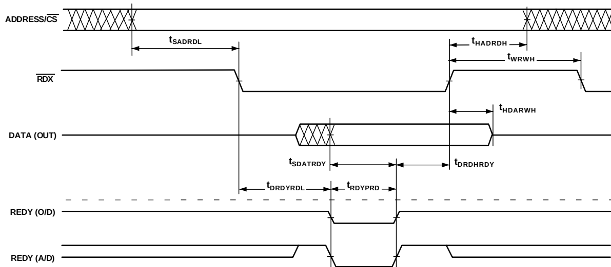
Figure 21. Read Cycle (Asynchronous Read—Host to ADSP-21160N)
