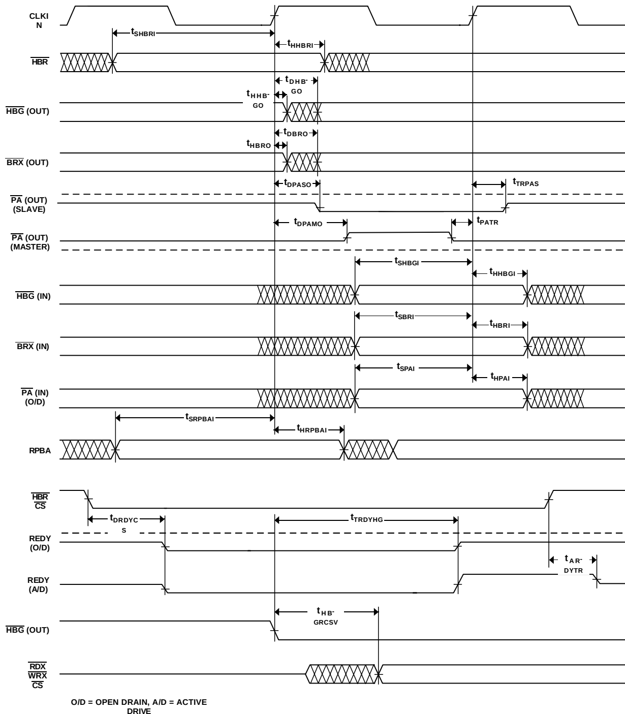
Figure 20. Multiprocessor Bus Request and Host Bus Request
