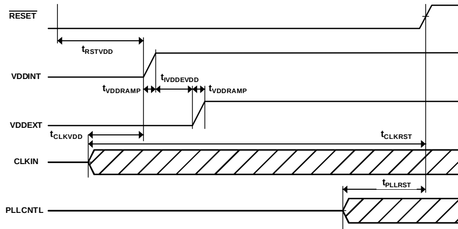
Figure 10. DSP Startup
