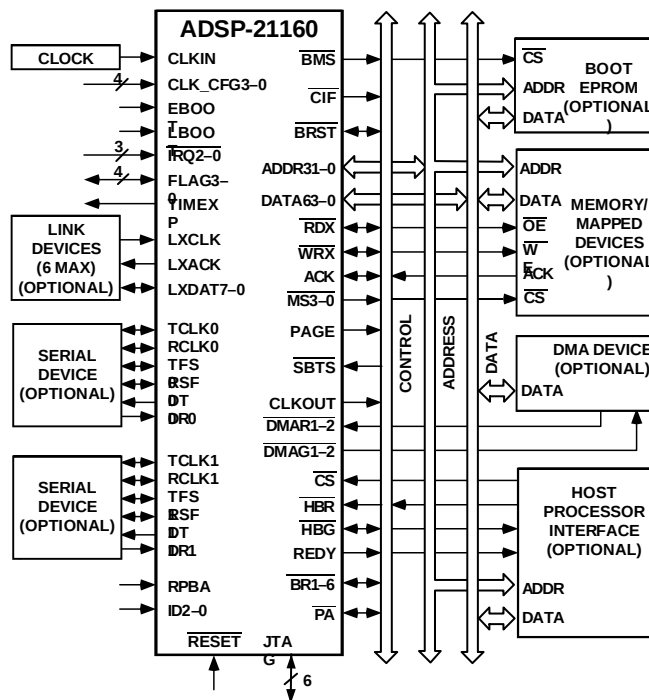
Figure 1. Single-Processor System
