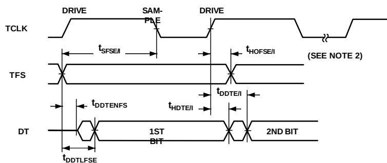
Figure 28. External Late Frame Sync
