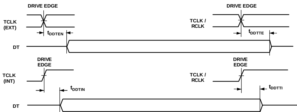
Figure 27. Serial Ports
