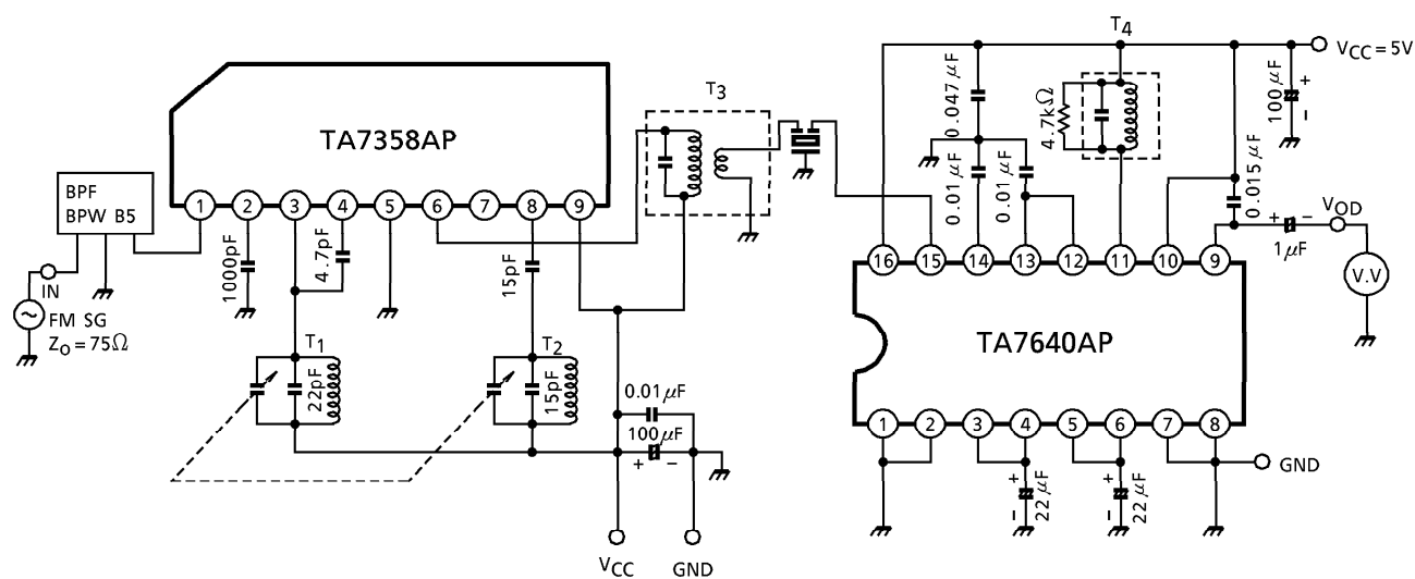
TEST CIRCUIT 2
