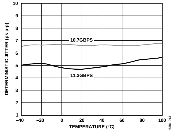
Figure 13. Deterministic Jitter vs. Temperature (Worse-Case Conditions, CPA Disabled)
