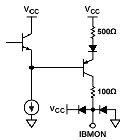
Figure 28. Equivalent Circuit of the IBMON Pin
