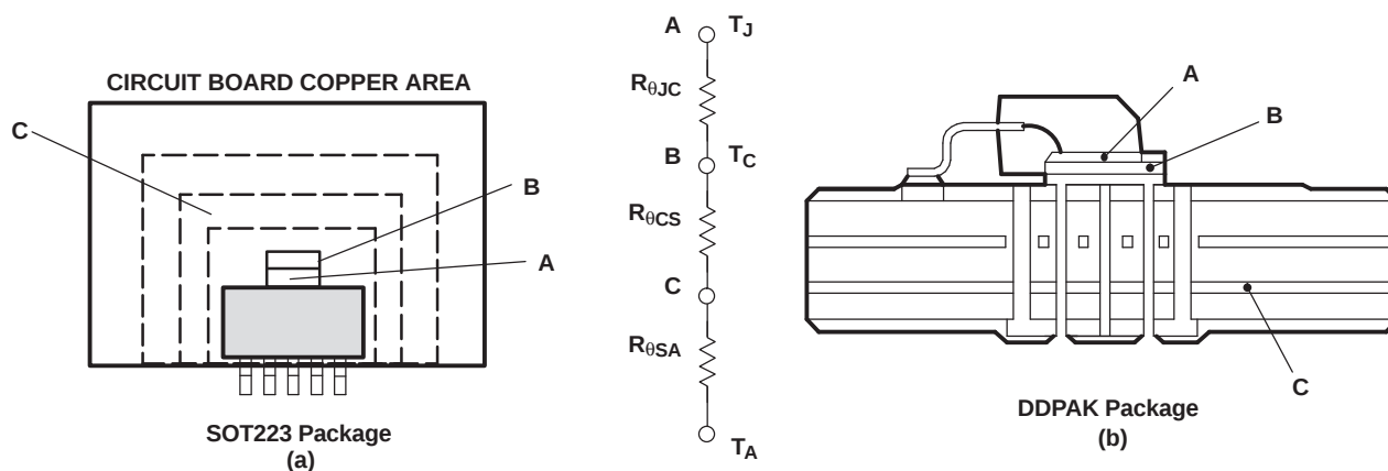
Figure 24. Thermal Resistances
