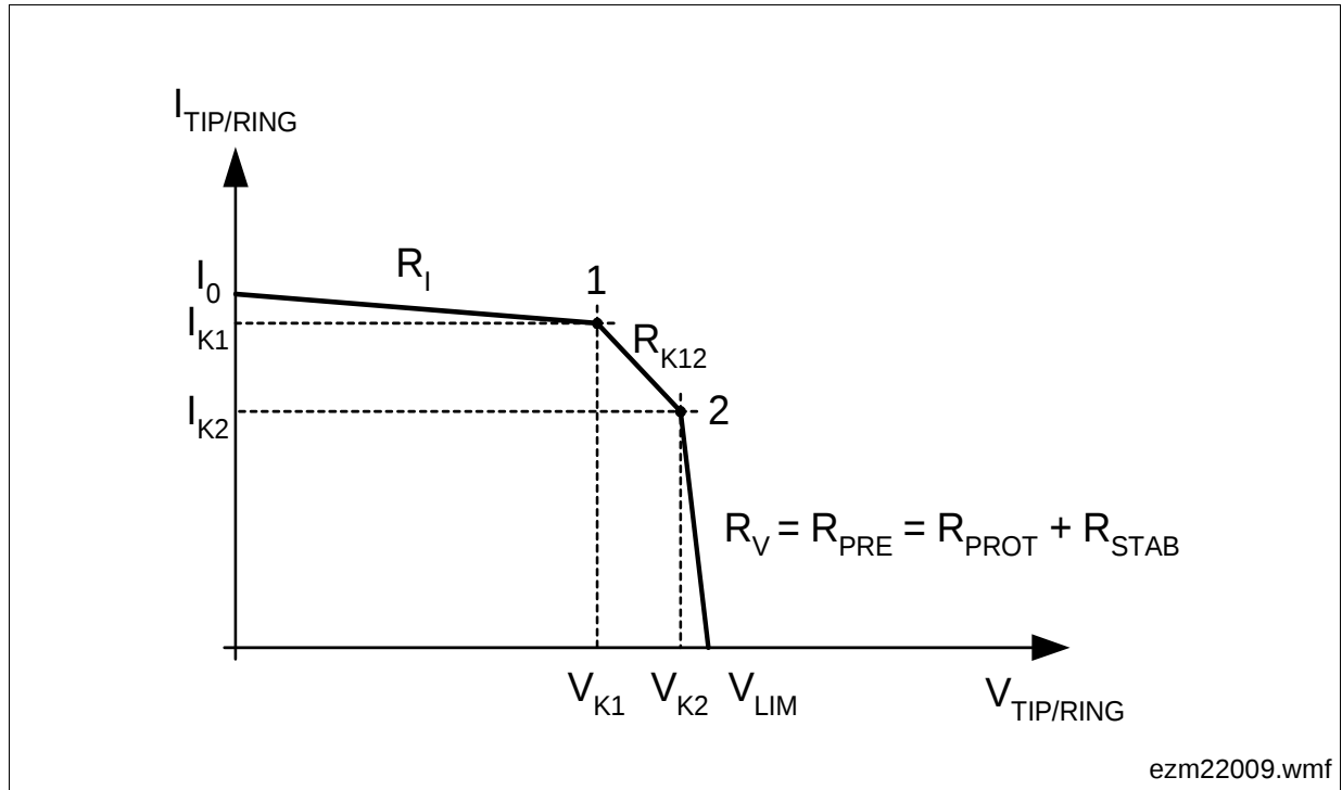
Figure 18 DC Characteristic
