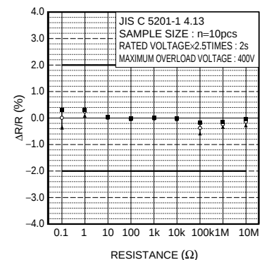
Fig.7 Overload
