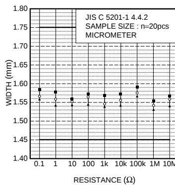
Fig.3 Dimensions (width)
