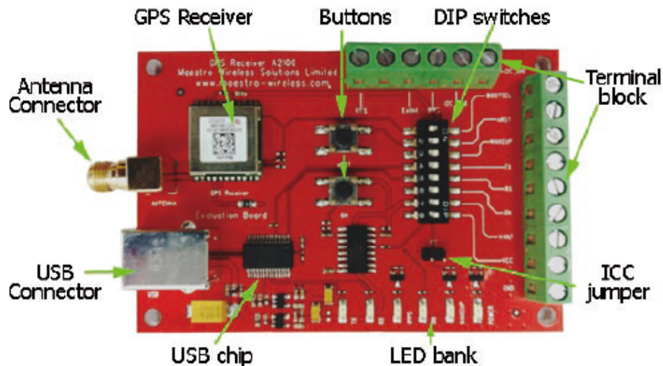
Figure 11: Board overview
