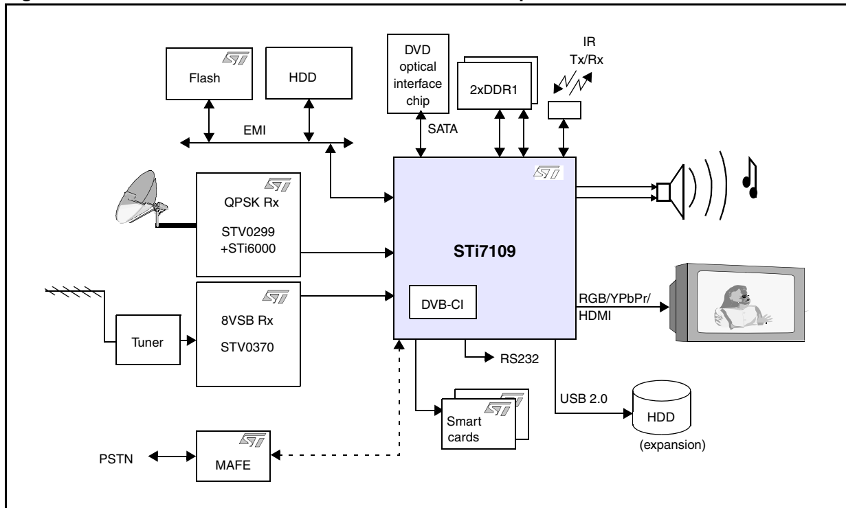
Figure 3. Low-cost dual satellite and terrestrial HD set-top box with HDD and DVD
