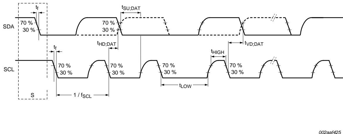
Fig 18. I 2 C-bus pins clock timing
