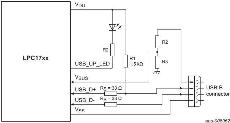
Fig 31. USB interface on a bus-powered device where VBUS = 5 V, VDD not present
